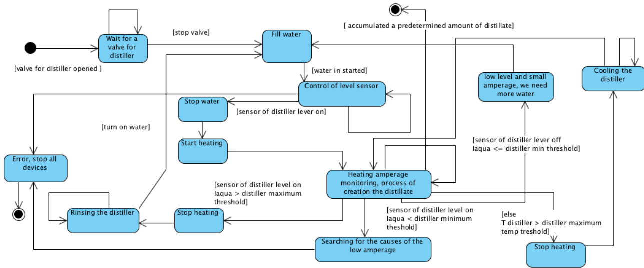
Fig. 3. State machine for water preparation
